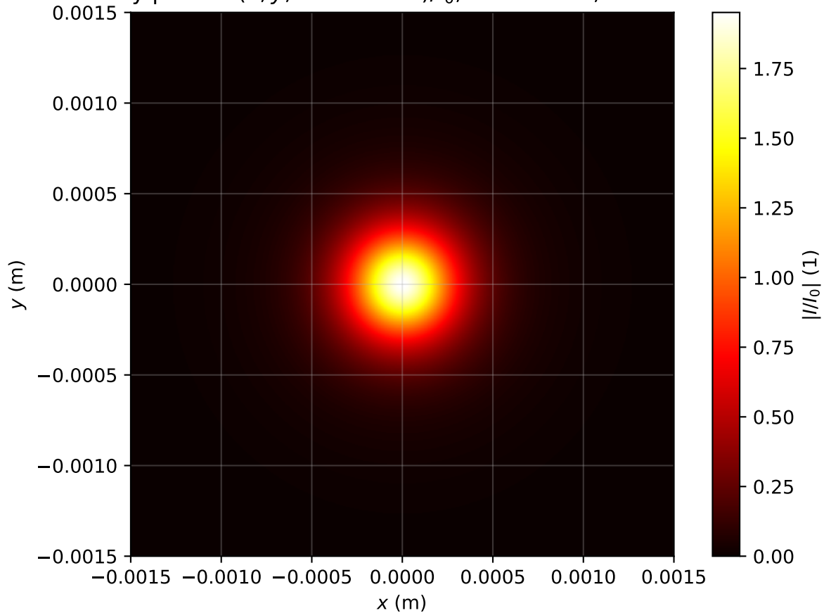
Intensity profile I(x, y, z = 1.672m)/I_0 , P_{in}=1.0P_{cr} , artificial time
